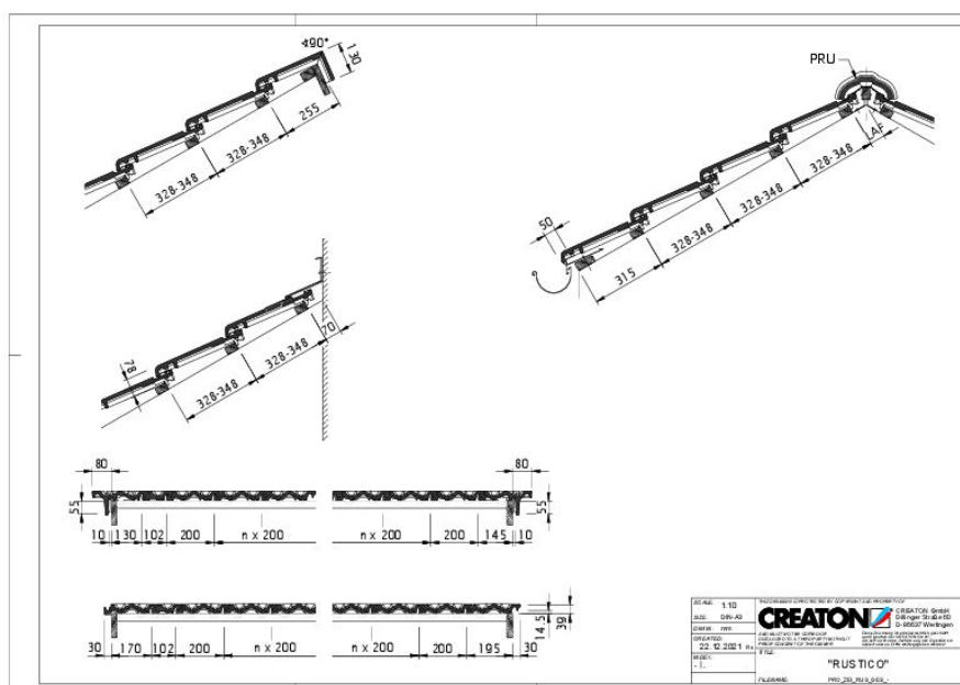
Drawing RUSTICO general view GES
